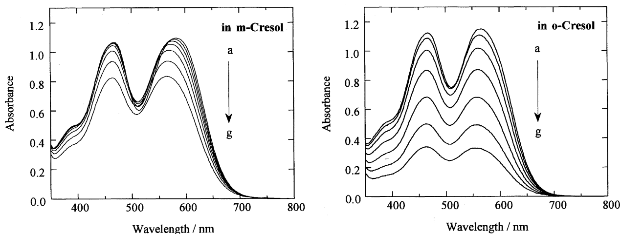
Fig. 4. Electronic absorption spectra of 1 ( 7.5 \times 10^{-5} M) in m -cresol and in o -cresol at various temperatures. The changes in the concentrations of 1 by solvent expansion with increasing temperature were corrected. Temperature: a, 20; b, 35; c, 50; d, 65; e, 80; f, 95; g, 110 °C. Light-path length: 1 cm.
